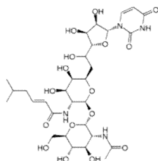
Tunicamycin
