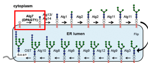
Glycan synthesis for protein N-glycosylation
